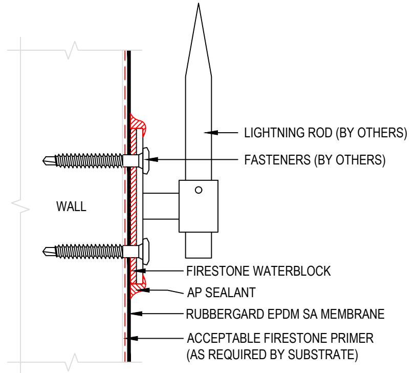
WALL MOUNT
