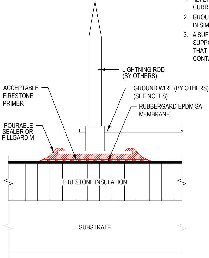
ROOF MOUNT
