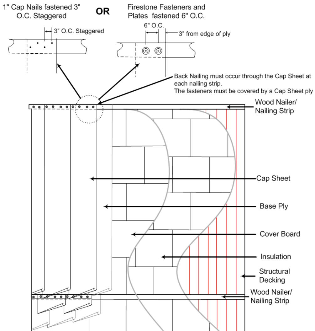
Figure 2: Back-nailing
