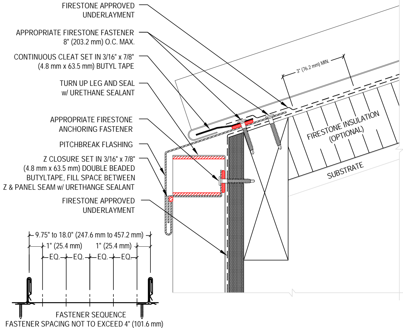
FASTENER SEQUENCE FASTENER SPACING NOT TO EXCEED 4" (101.6 mm) ANCHORING FASTENER PATTERN
