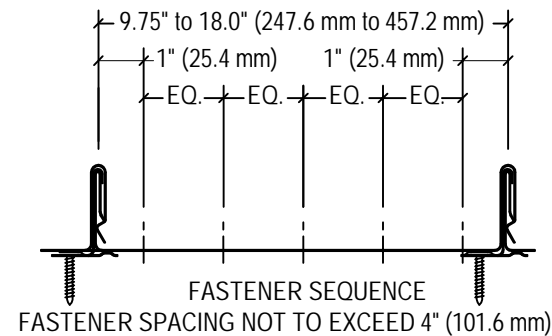
FASTENER SEQUENCE FASTENER SPACING NOT TO EXCEED 4" (101.6 mm) ANCHORING FASTENER PATTERN
